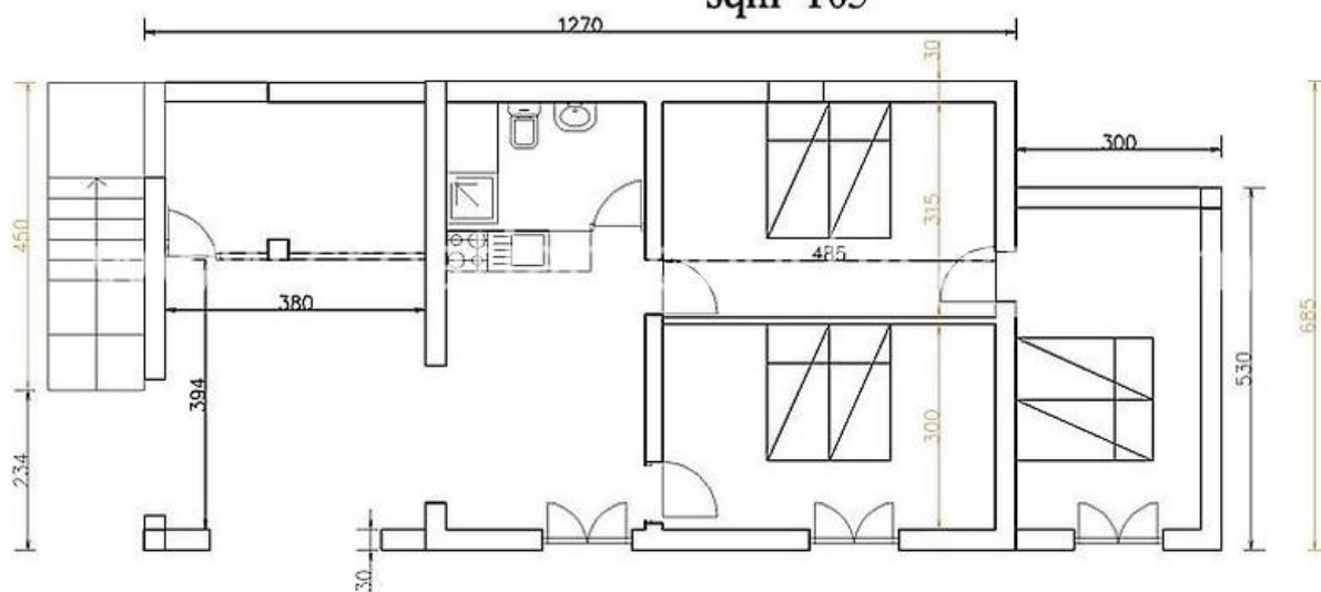
ground floor 2013 sqm 105
